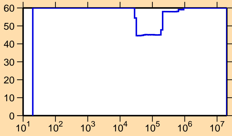
\Delta\sigma/\sigma vs. E for ^{175}\text{Ta}(n,\gamma)
