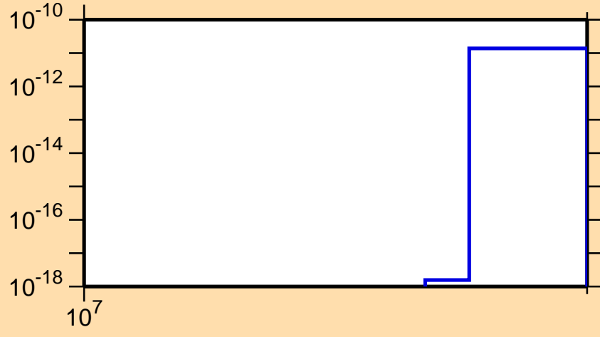
\sigma vs. E for ^{175}\text{Ta}(n,3n\alpha)
