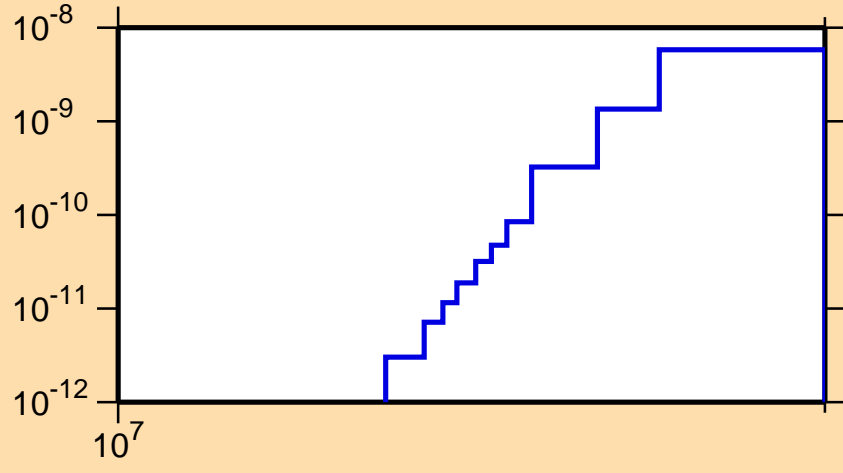
\sigma vs. E for ^{175}\text{Ta} (mt 45)
