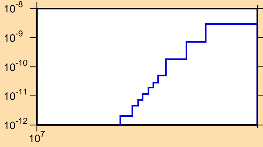
\sigma vs. E for ^{175}\text{Ta}(\text{mt117})
