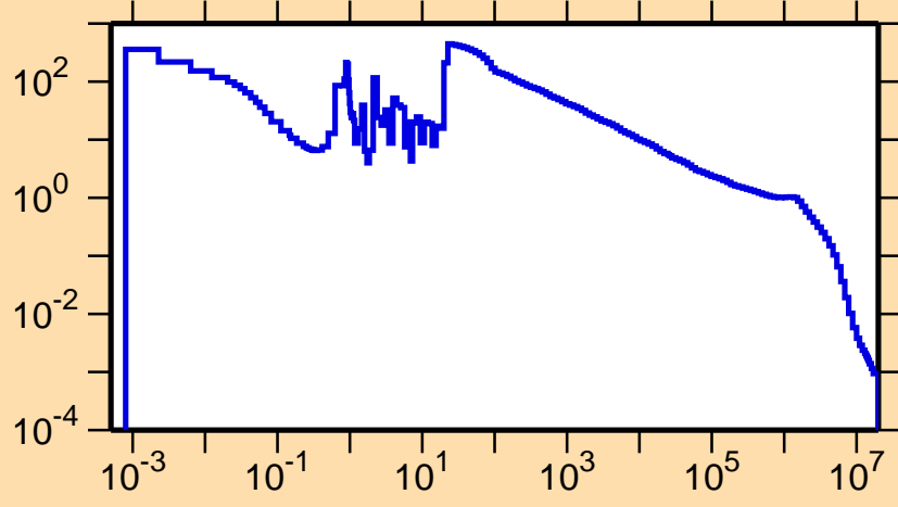
\sigma vs. E for ^{175}\text{Ta}(n,\gamma)
