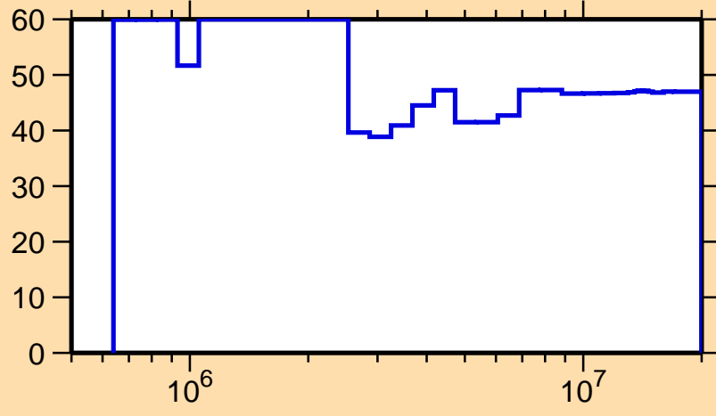
\Delta\sigma/\sigma vs. E for ^{175}\text{Ta}(n,n_1)
