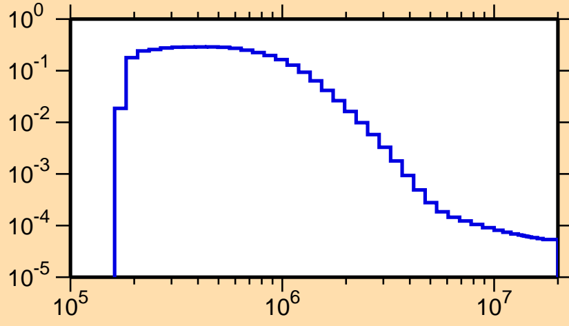
\sigma vs. E for ^{177}\text{Ta}(n,n_4)
