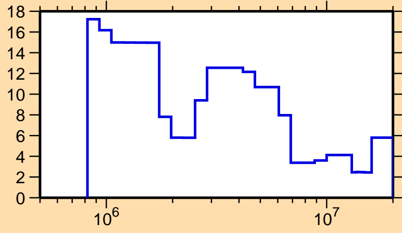
\Delta\sigma/\sigma vs. E for ^{177}\text{Ta}(n,tot.)
