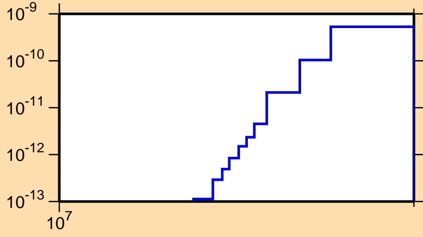
\sigma vs. E for ^{177}\text{Ta}(\text{mt117})
