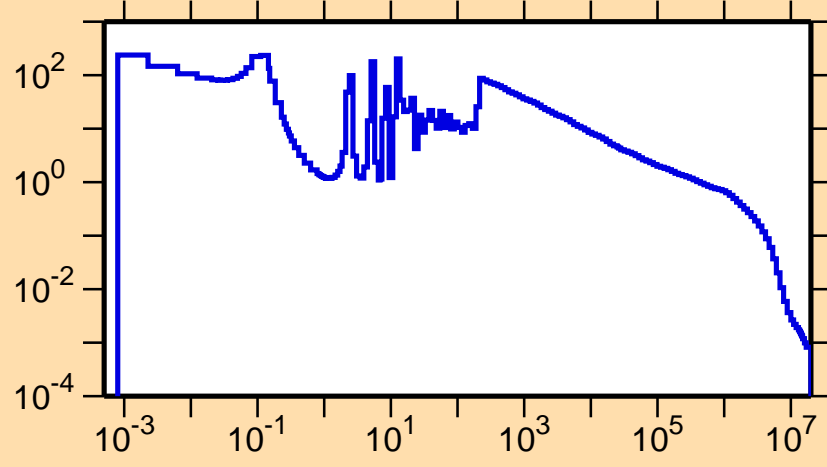
\sigma vs. E for ^{177}\text{Ta}(n,\gamma)
