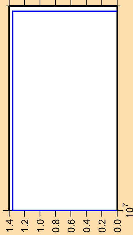
\Delta\sigma/\sigma vs. E for ^{177}\text{Ta}(n,3n\alpha)
