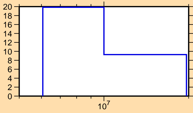
\Delta\sigma/\sigma vs. E for ^{177}\text{Ta}(n,2n)
