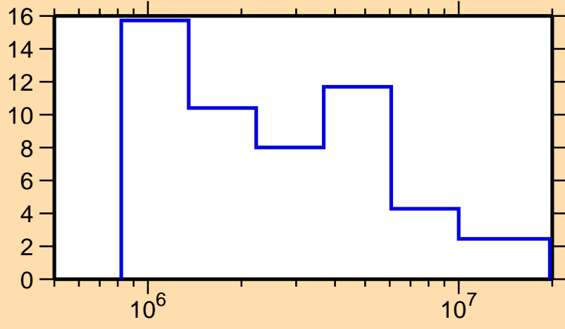
\Delta\sigma/\sigma vs. E for ^{177}\text{Ta}(n,tot.)
