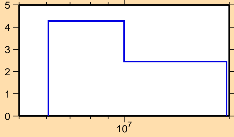
\Delta\sigma/\sigma vs. E for ^{177}\text{Ta}(n,\text{tot.})
