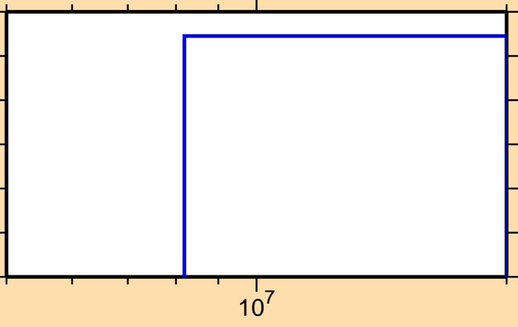
\sigma vs. E for ^{177}\text{Ta}(n,2np)
