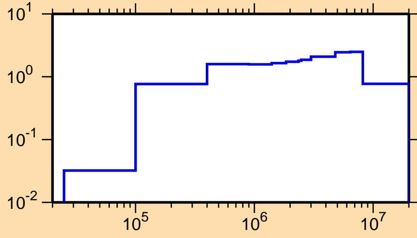
\sigma vs. E for ^{177}\text{Ta}(n,\text{inel.})
