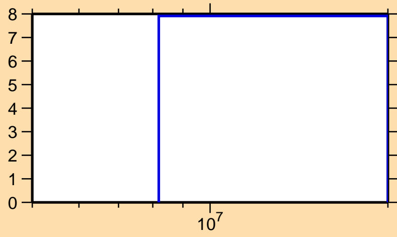
\Delta\sigma/\sigma vs. E for ^{177}\text{Ta}(n,\text{nonel.})
