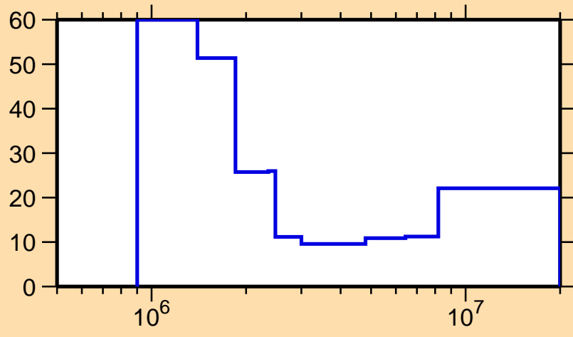
\Delta\sigma/\sigma vs. E for ^{177}\text{Ta}(n,n\text{cont.})
