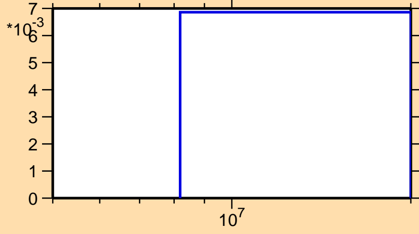
\sigma vs. E for ^{177}\text{Ta}(n,3n)
