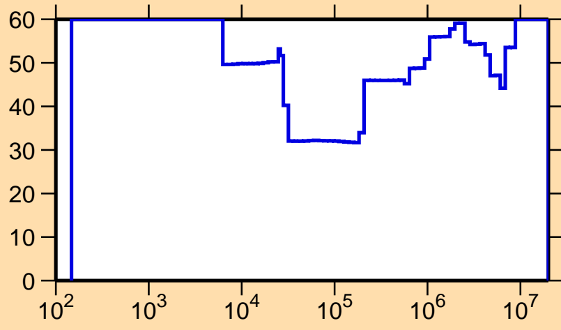
\Delta\sigma/\sigma vs. E for ^{178}\text{Ta}(n,\gamma)
