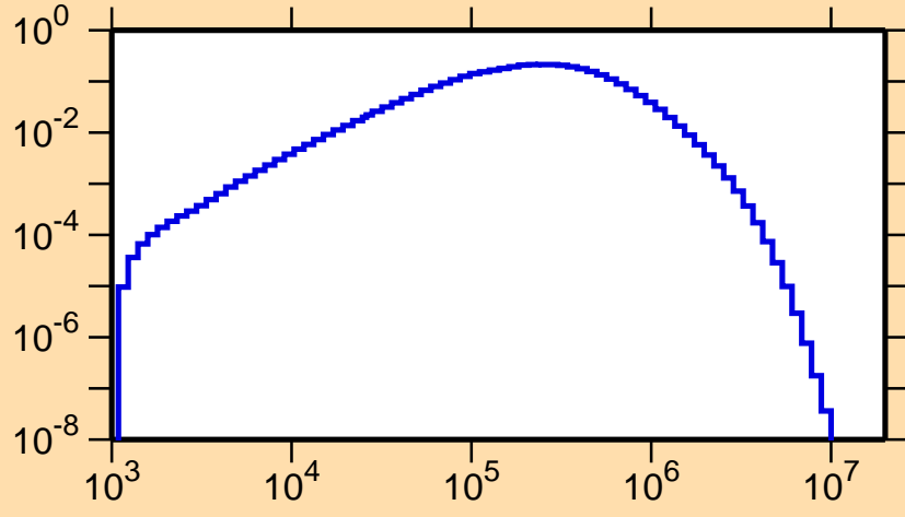
\sigma vs. E for ^{178}\text{Ta}(n,n_2)
