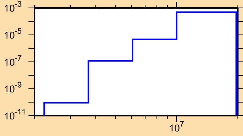
\sigma vs. E for ^{178}\text{Ta}(n,n\alpha)
