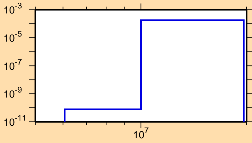
\sigma vs. E for ^{178}\text{Ta}(n,t)
