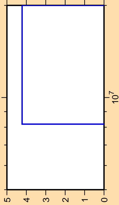
\Delta\sigma/\sigma vs. E for ^{178}\text{Ta}(n,3n\alpha)
