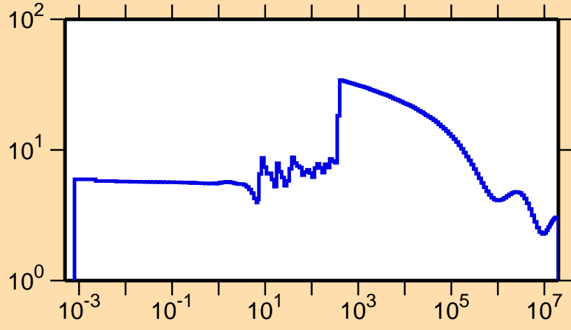
\sigma vs. E for ^{179}\text{Ta}(n,\text{el.})
