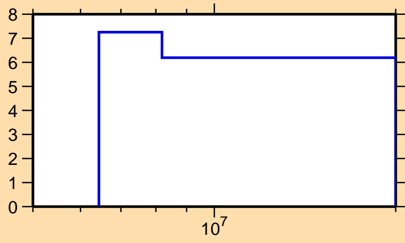
\Delta\sigma/\sigma vs. E for ^{179}\text{Ta}(n,\text{nonel.})
