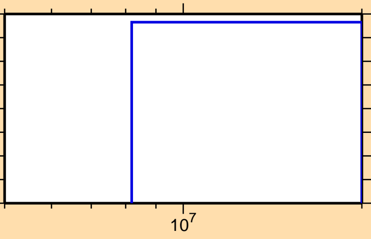
\sigma vs. E for ^{179}\text{Ta}(n,2np)
