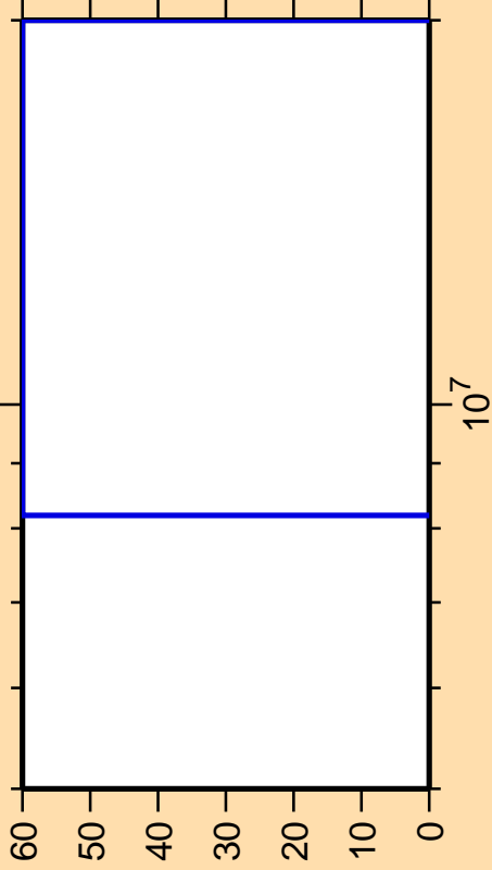
\Delta\sigma/\sigma vs. E for ^{179}\text{Ta}(n,\text{nd})
