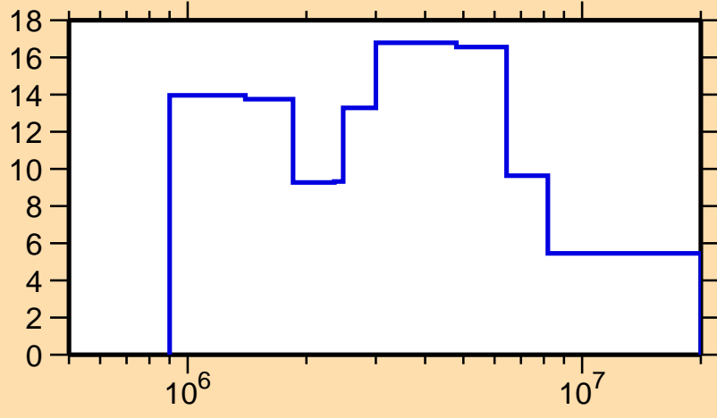
\Delta\sigma/\sigma vs. E for ^{179}\text{Ta}(n,el.)
