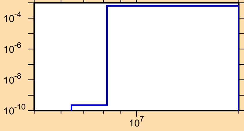
\sigma vs. E for ^{179}\text{Ta}(n,np)
