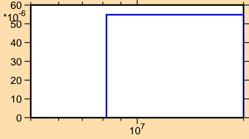
\sigma vs. E for ^{179}\text{Ta}(n,t)
