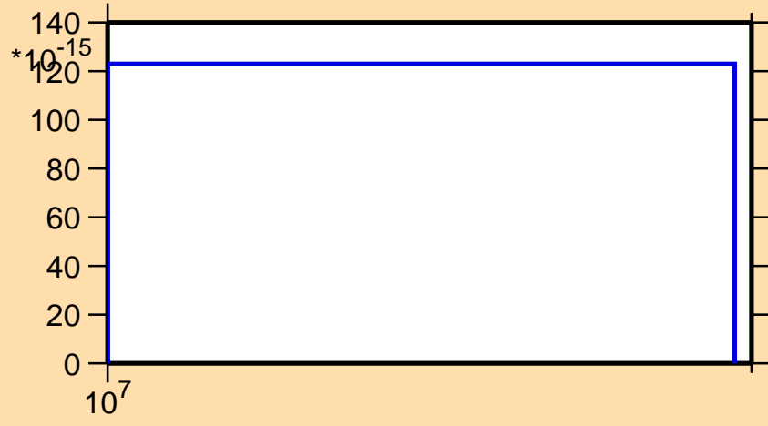
\sigma vs. E for ^{180}\text{Ta} (mt 45)
