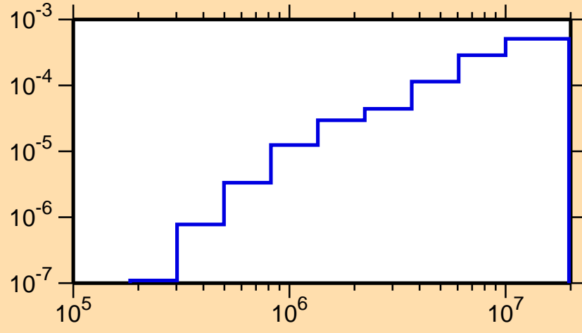
\sigma vs. E for ^{180}\text{Ta}(n,n_2)
