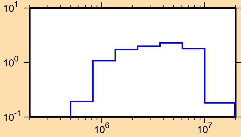
\sigma vs. E for ^{180}\text{Ta}(n,n\text{cont.})
