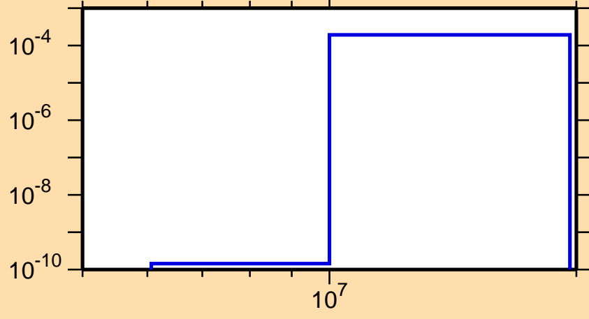
\sigma vs. E for ^{180}\text{Ta}(n,t)
