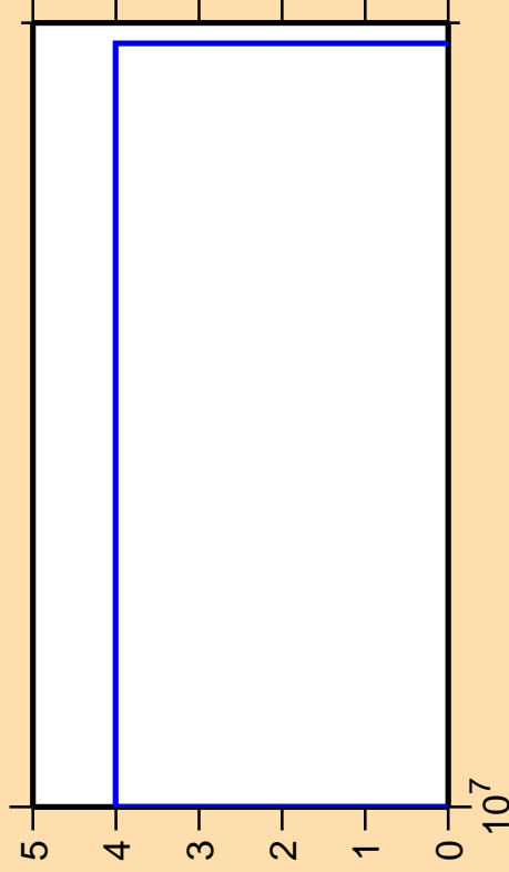
\Delta\sigma/\sigma vs. E for ^{180}\text{Ta}(\text{mt117})
