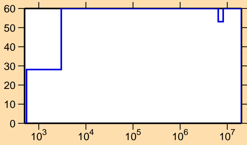
\Delta\sigma/\sigma vs. E for ^{180}\text{Ta}(n,\gamma)
