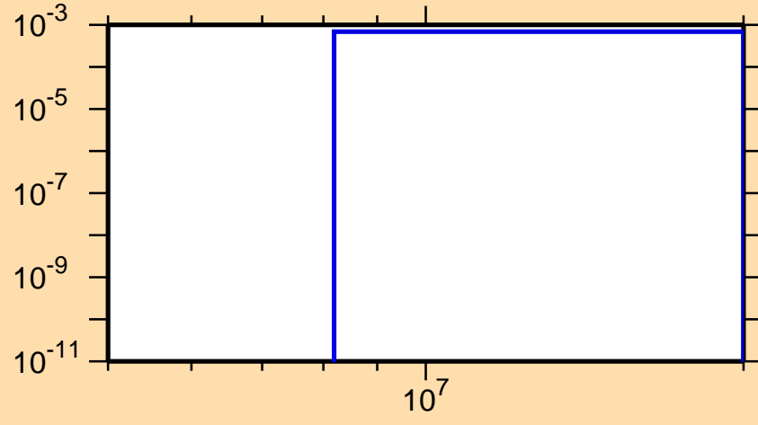
\sigma vs. E for ^{180}\text{Ta}(n,np)
