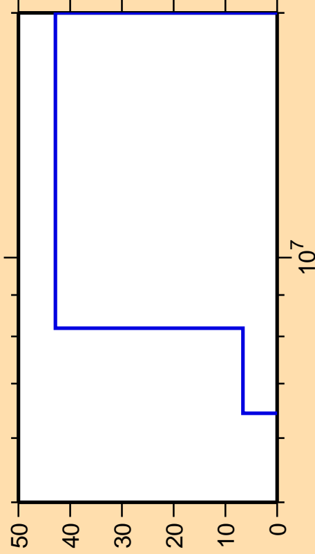
\Delta\sigma/\sigma vs. E for ^{180}\text{Ta}(n,np)
