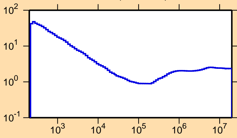
\sigma vs. E for ^{180}\text{Ta}(n,\text{nonel.})
