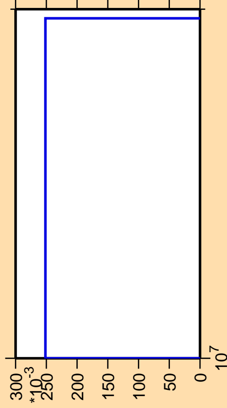
\Delta\sigma/\sigma vs. E for ^{180}\text{Ta} (mt 45)
