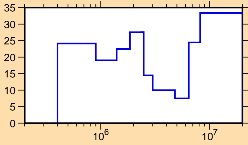
\Delta\sigma/\sigma vs. E for ^{180}\text{Ta}(n,n\text{cont.})
