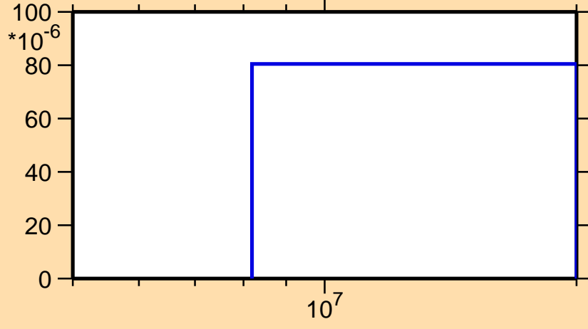
\sigma vs. E for ^{180}\text{Ta}(n,t)
