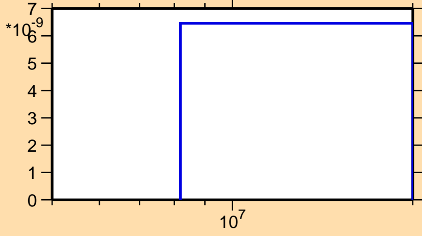
\sigma vs. E for ^{180}\text{Ta}(n,nt)
