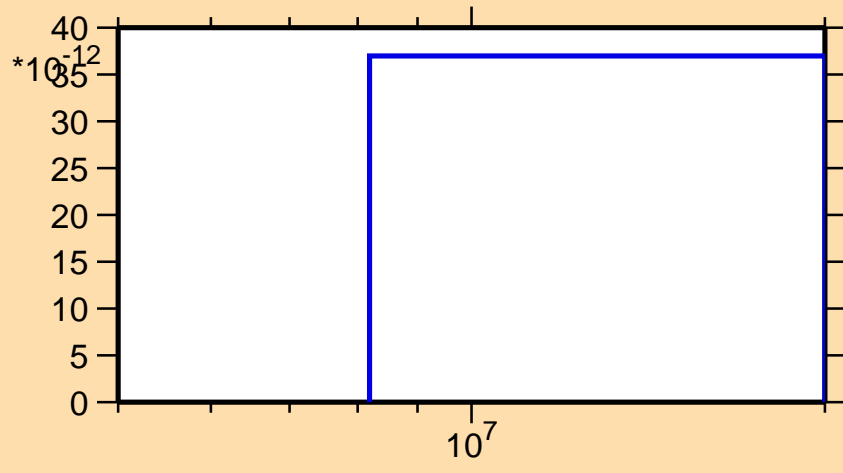
\sigma vs. E for ^{180}\text{Ta}(n,\text{He}3)
