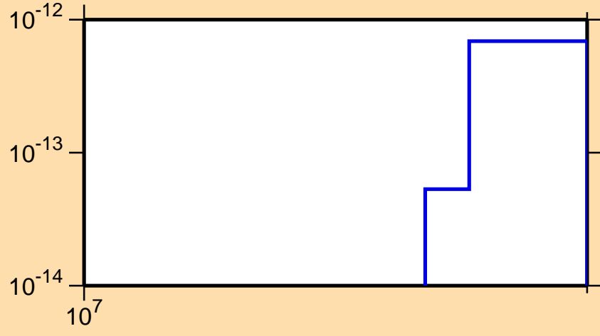
\sigma vs. E for ^{181}\text{Ta}(\text{mt117})
