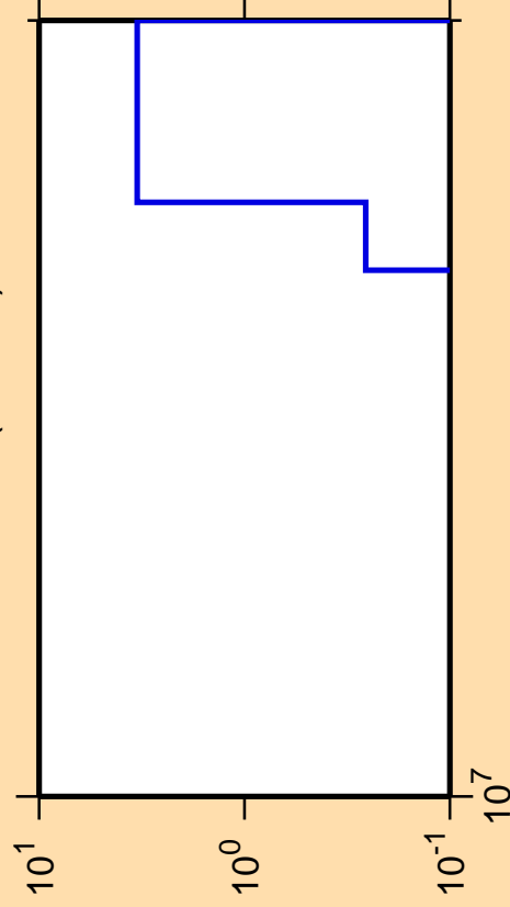
\Delta\sigma/\sigma vs. E for ^{181}\text{Ta}(\text{mt117})
