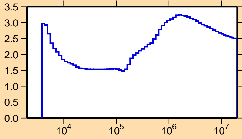
\sigma vs. E for ^{181}\text{Ta}(n,\text{nonel.})
