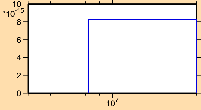
\sigma vs. E for ^{181}\text{Ta}(\text{mt117})
