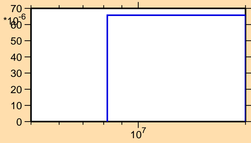
\sigma vs. E for ^{181}\text{Ta}(n,t)
