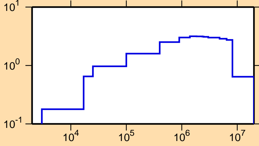
\sigma vs. E for ^{181}\text{Ta}(n,\text{inel.})
