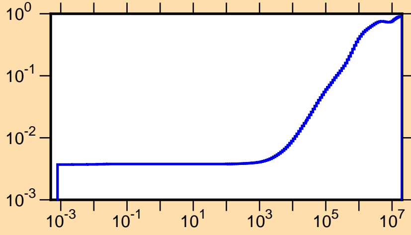
\mu vs. E for ^{182}\text{Ta}(\text{mt251})
