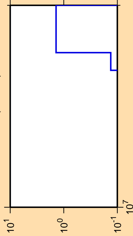
\Delta\sigma/\sigma vs. E for ^{182}\text{Ta}(\text{mt117})
