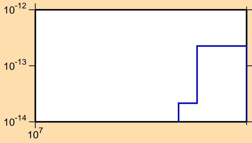
\sigma vs. E for ^{182}\text{Ta}(\text{mt117})
