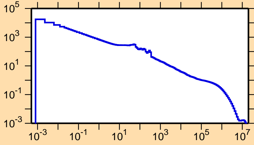
\sigma vs. E for ^{182}\text{Ta}(n,\gamma)
