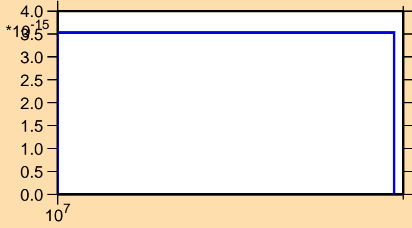
\sigma vs. E for ^{182}\text{Ta} (mt117)
