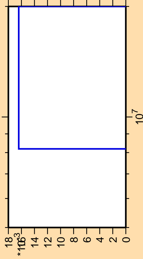
\Delta\sigma/\sigma vs. E for ^{182}\text{Ta}(\text{mt117})
