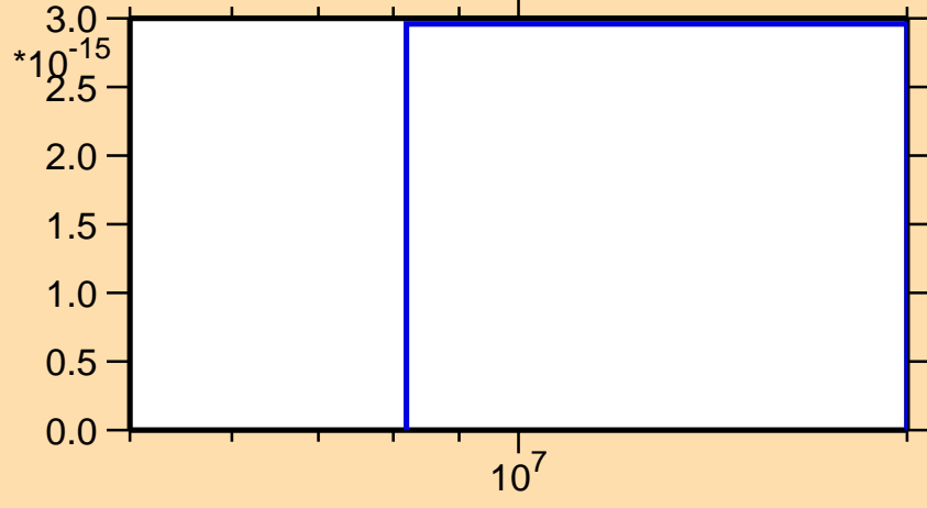
\sigma vs. E for ^{182}\text{Ta}(\text{mt117})
