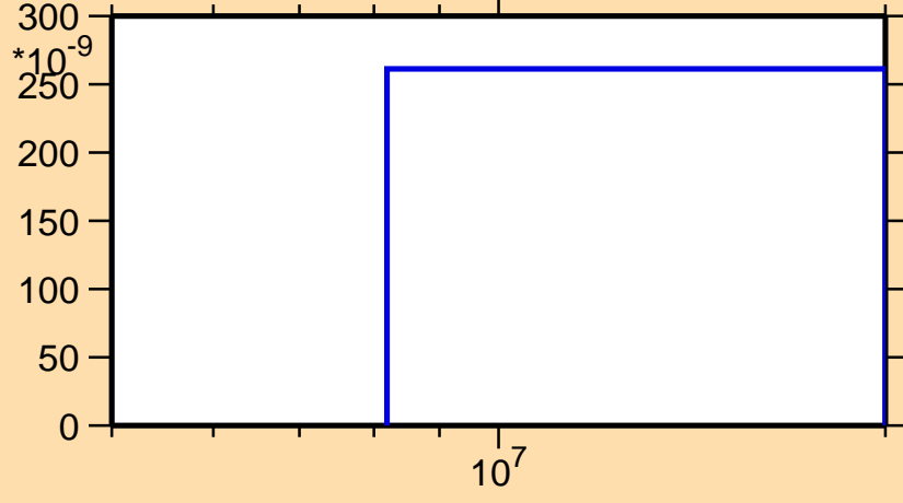
\sigma vs. E for ^{182}\text{Ta}(n,2n\alpha)
