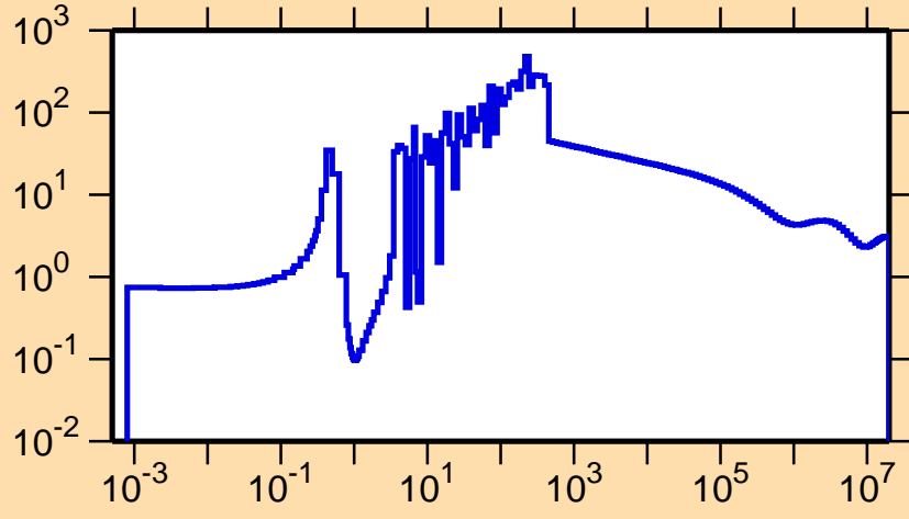
\sigma vs. E for ^{183}\text{Ta}(n,\text{el.})
