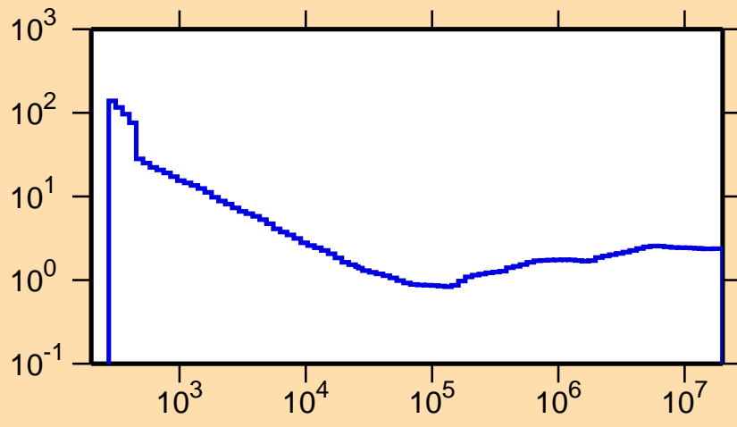
\sigma vs. E for ^{183}\text{Ta}(n,\text{nonel.})
