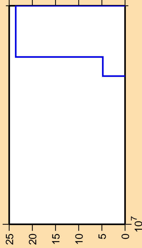
\Delta\sigma/\sigma vs. E for ^{183}\text{Ta}(n,p\alpha)
