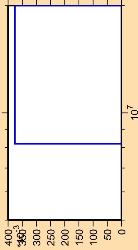
\Delta\sigma/\sigma vs. E for ^{183}\text{Ta}(n,p\alpha)
