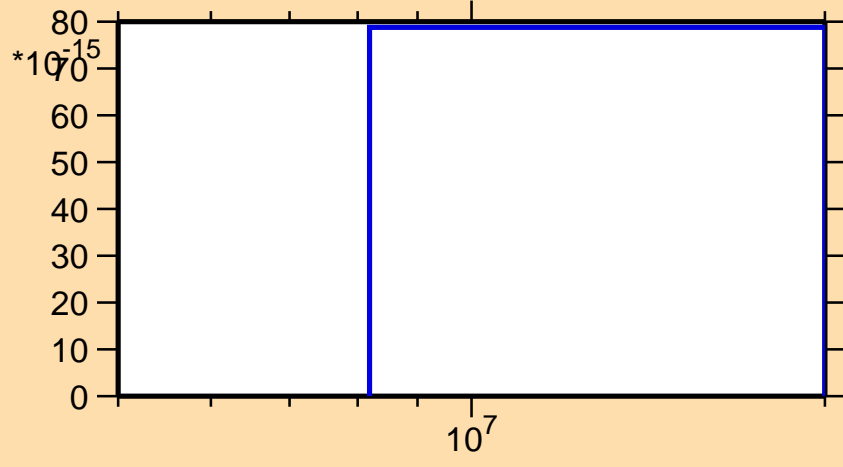
\sigma vs. E for ^{183}\text{Ta}(n,p\alpha)
