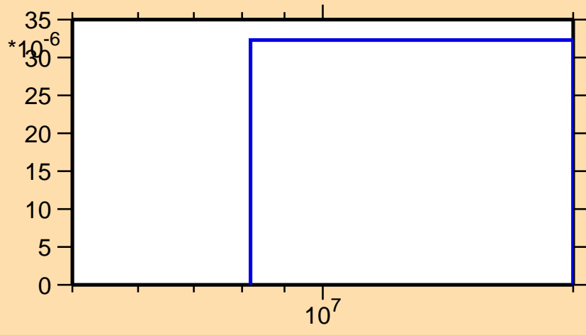
\sigma vs. E for ^{183}\text{Ta}(n,t)
