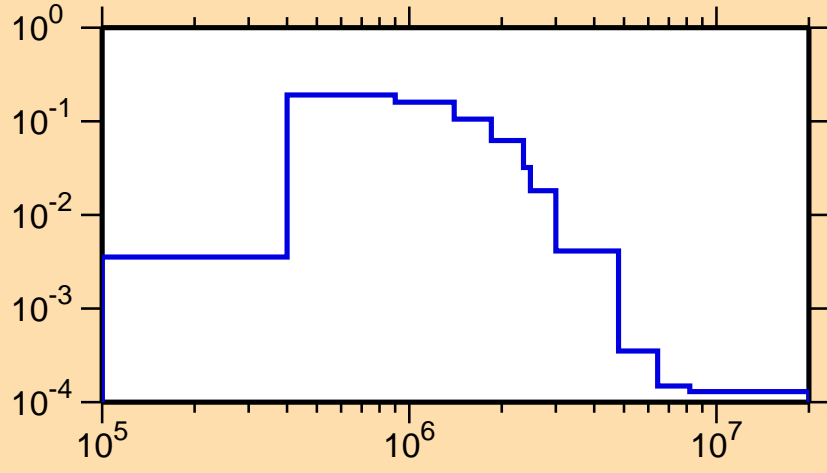
\sigma vs. E for ^{183}\text{Ta}(n,n_3)
