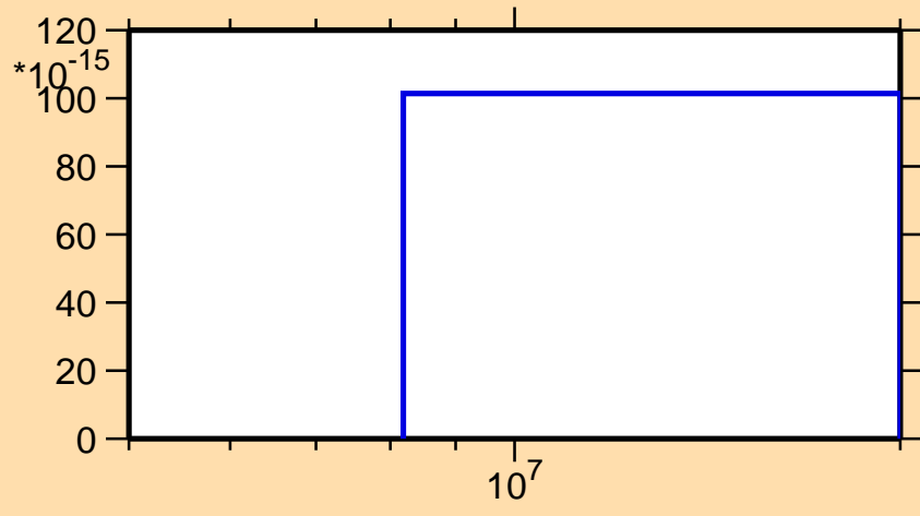
\sigma vs. E for ^{183}\text{Ta}(n,3n\alpha)
