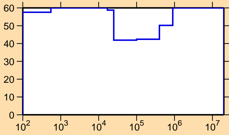
\Delta\sigma/\sigma vs. E for ^{184}\text{Ta}(n,\gamma)
