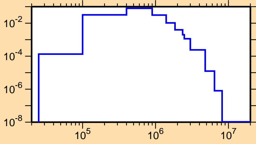
\sigma vs. E for ^{184}\text{Ta}(n,n_2)
