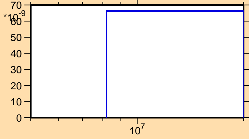
\sigma vs. E for ^{184}\text{Ta}(n,2n\alpha)
