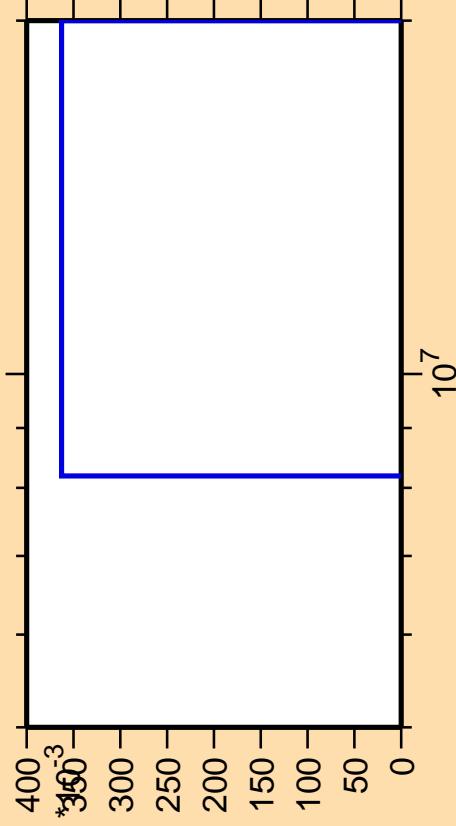
\Delta\sigma/\sigma vs. E for ^{184}\text{Ta}(n,\text{He}3)
