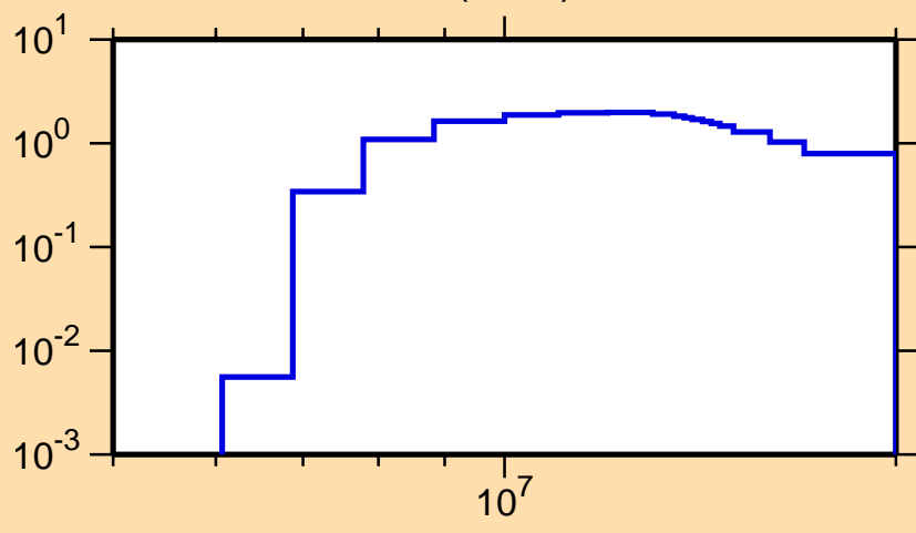
\sigma vs. E for ^{185}\text{Ta}(n,2n)
