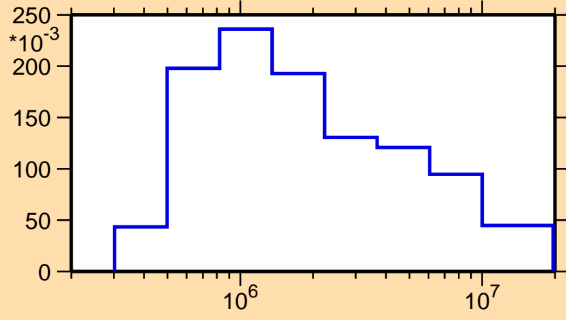
\sigma vs. E for ^{185}\text{Ta}(n,n_3)
