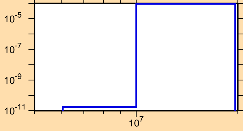
\sigma vs. E for ^{185}\text{Ta}(n,d)
