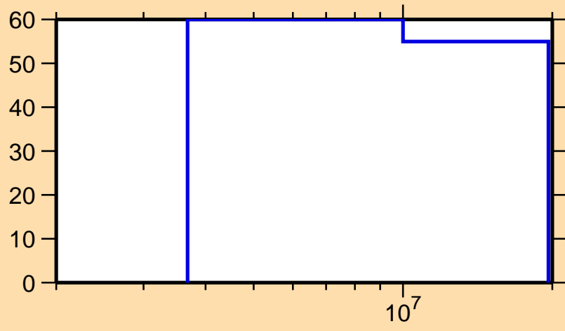
\Delta\sigma/\sigma vs. E for ^{185}\text{Ta}(n,p)
