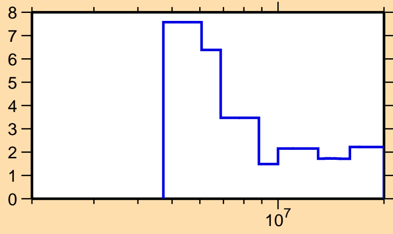
\Delta\sigma/\sigma vs. E for ^{186}\text{Ta}(n,\text{tot.})
