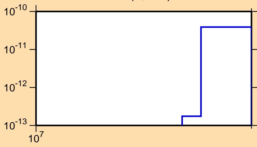
\sigma vs. E for ^{186}\text{Ta}(n,3n\alpha)
