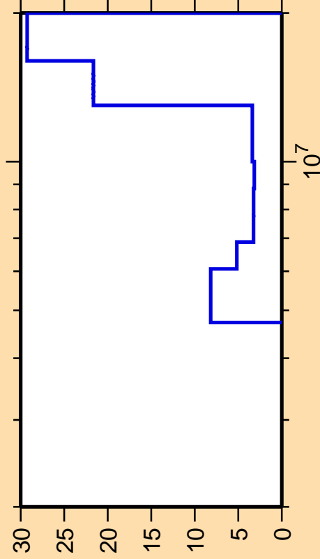
\Delta\sigma/\sigma vs. E for ^{186}\text{Ta}(n,2n)
