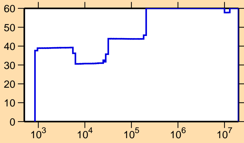
\Delta\sigma/\sigma vs. E for ^{186}\text{Ta}(n,\gamma)
