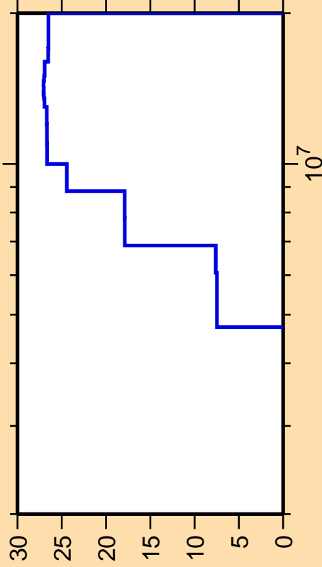
\Delta\sigma/\sigma vs. E for ^{186}\text{Ta}(n,n\text{cont.})
