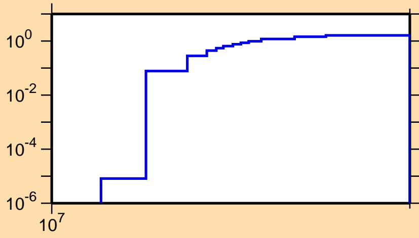
\sigma vs. E for ^{186}\text{Ta}(n,3n)
