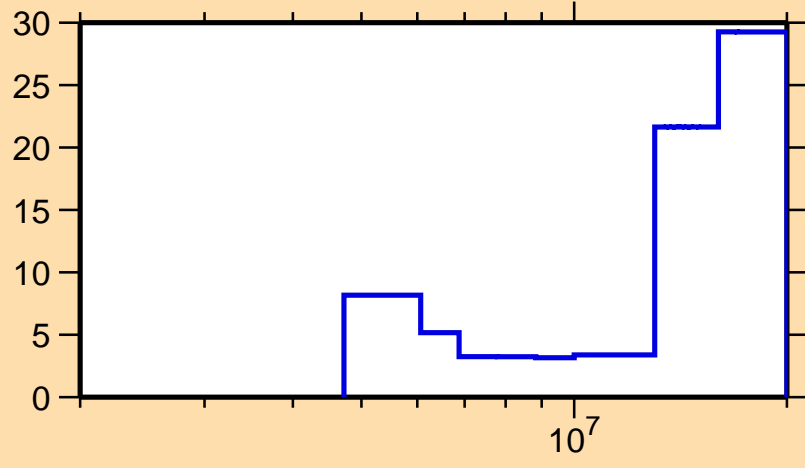
\Delta\sigma/\sigma vs. E for ^{186}\text{Ta}(n,2n)
