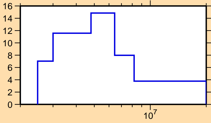
\Delta\sigma/\sigma vs. E for ^{186}\text{Ta}(n,el.)
