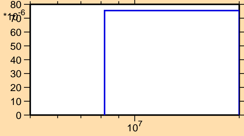
\sigma vs. E for ^{186}\text{Ta}(n,d)
