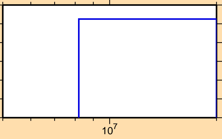
\sigma vs. E for ^{186}\text{Ta}(n,\text{He3})
