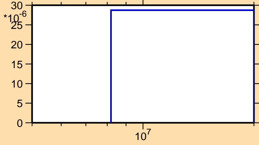
\sigma vs. E for ^{186}\text{Ta}(n,t)
