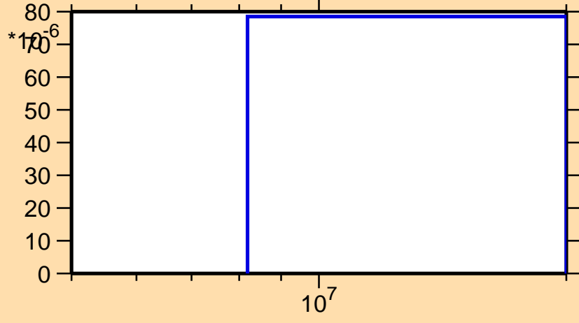
\sigma vs. E for ^{186}\text{Ta}(n,np)
