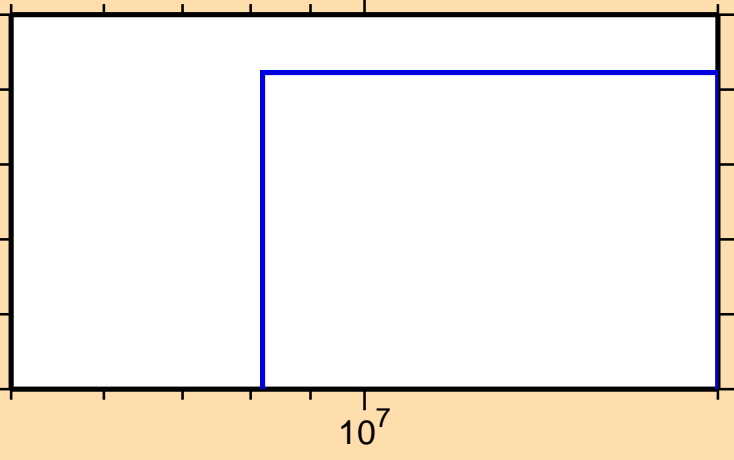
\sigma vs. E for ^{186}\text{Ta}(n,\text{nd})
