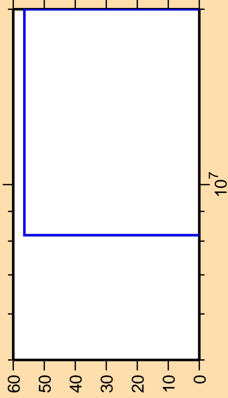
\Delta\sigma/\sigma vs. E for ^{186}\text{Ta}(n,np)
