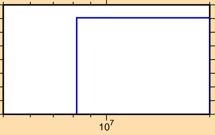
\sigma vs. E for ^{186}\text{Ta}(n,nt)
