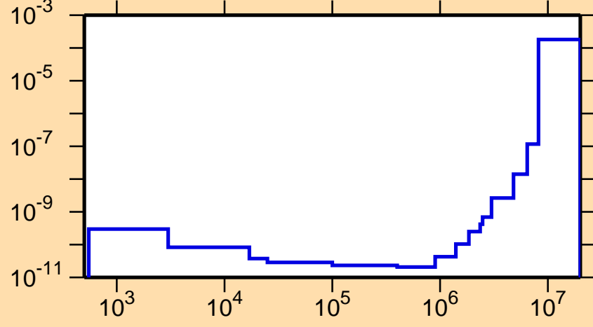
\sigma vs. E for ^{186}\text{Ta}(n,\alpha)
