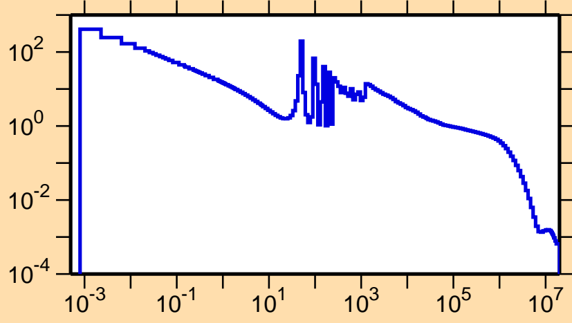
\sigma vs. E for ^{188}\text{Ta}(n,\gamma)
