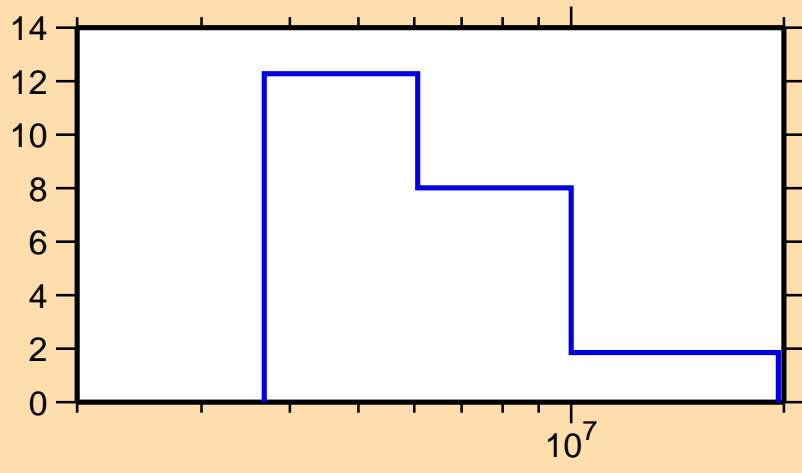
\Delta\sigma/\sigma vs. E for ^{188}\text{Ta}(n,\text{tot.})
