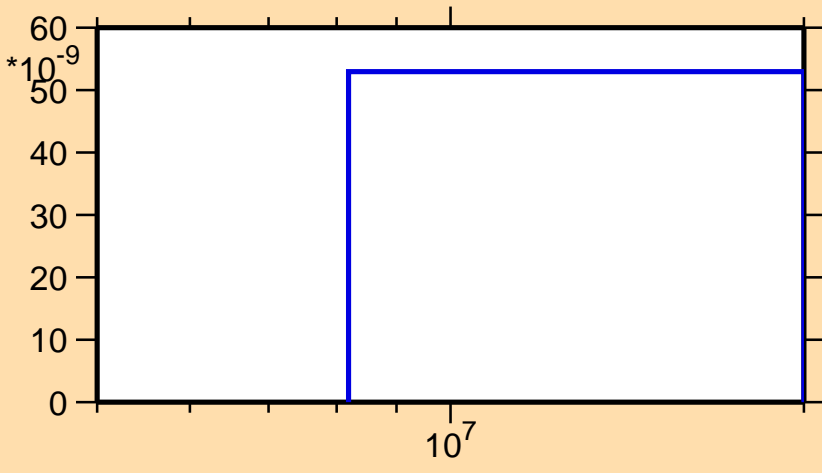
\sigma vs. E for ^{188}\text{Ta}(n,nt)
