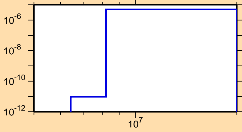
\sigma vs. E for ^{188}\text{Ta}(n,n\alpha)
