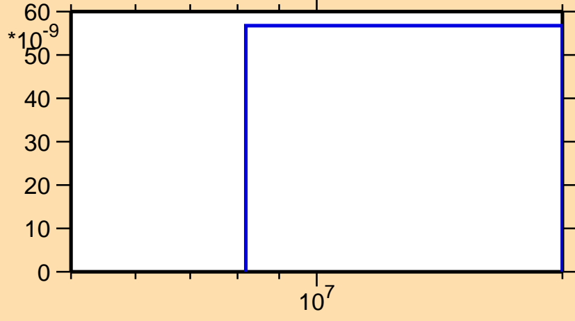
\sigma vs. E for ^{188}\text{Ta}(n,\text{nd})
