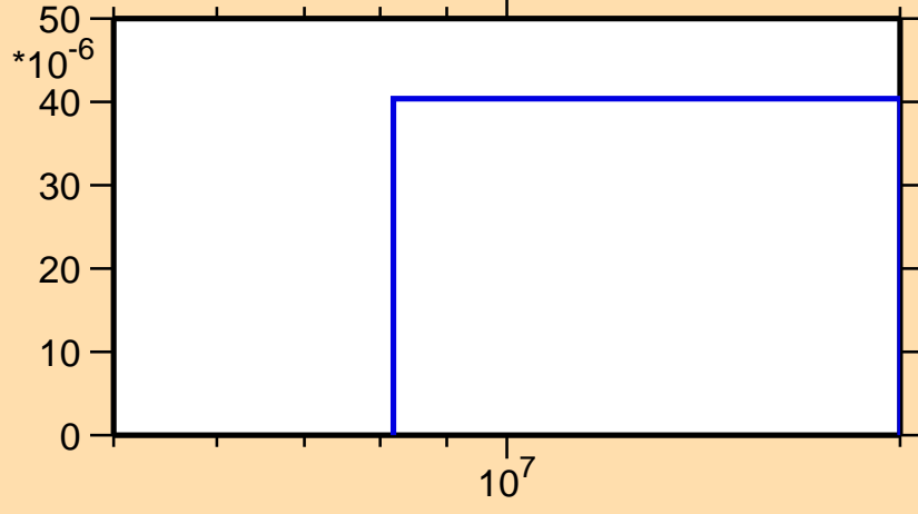
\sigma vs. E for ^{188}\text{Ta}(n,d)
