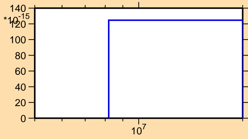
\sigma vs. E for ^{188}\text{Ta}(n,3n\alpha)
