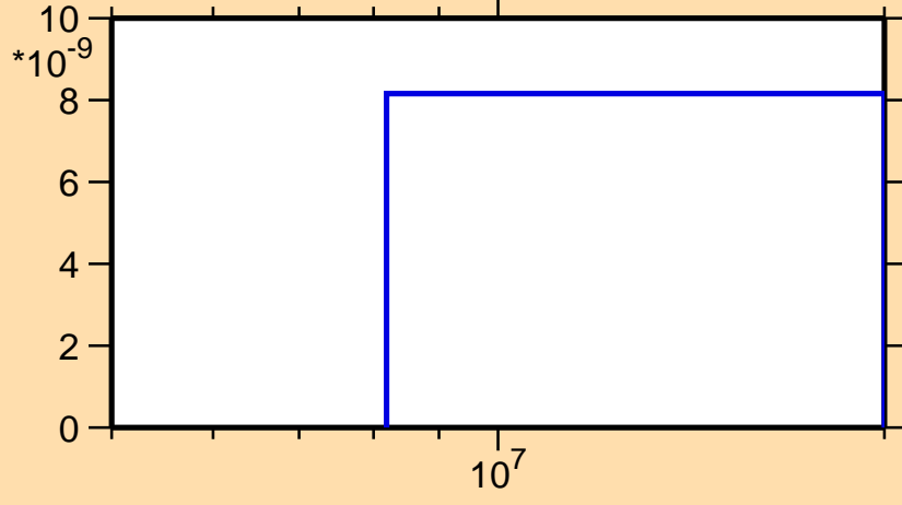
\sigma vs. E for ^{188}\text{Ta}(n,2np)
