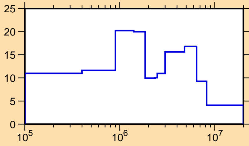
\Delta\sigma/\sigma vs. E for ^{188}\text{Ta}(n,\text{el.})
