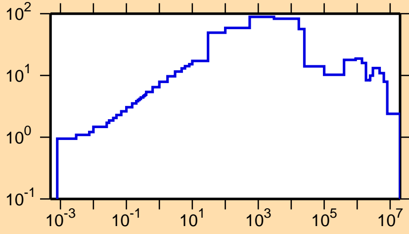
\Delta\sigma/\sigma vs. E for ^{188}\text{Ta}(n,\text{tot.})
