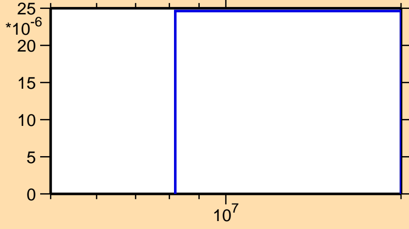
\sigma vs. E for ^{188}\text{Ta}(n,np)
