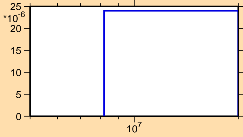
\sigma vs. E for ^{188}\text{Ta}(n,t)
