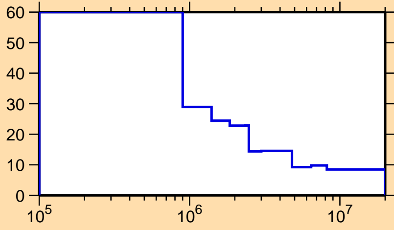
\Delta\sigma/\sigma vs. E for ^{188}\text{Ta}(n,\text{nonel.})
