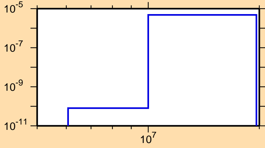
\sigma vs. E for ^{189}\text{Ta}(n,n\alpha)
