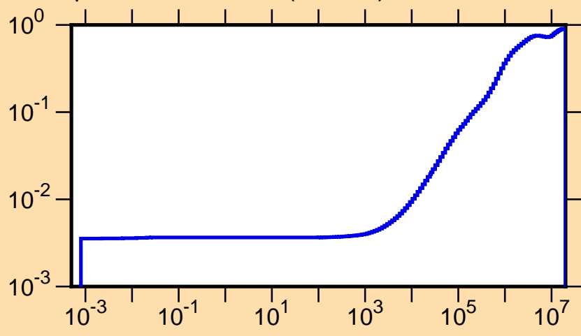
\mu vs. E for ^{190}\text{Ta}(\text{mt251})
