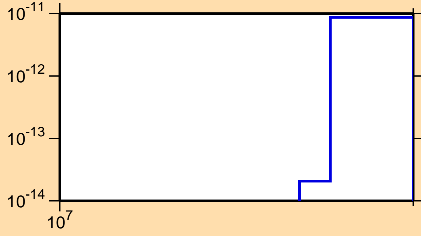
\sigma vs. E for ^{190}\text{Ta}(n,3n\alpha)
