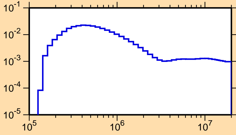
\sigma vs. E for ^{190}\text{Ta}(n,n_1)
