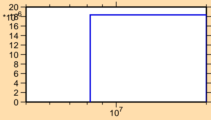
\sigma vs. E for ^{190}\text{Ta}(n,np)
