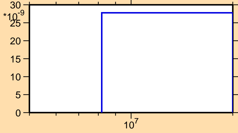
\sigma vs. E for ^{190}\text{Ta}(n,\text{nd})
