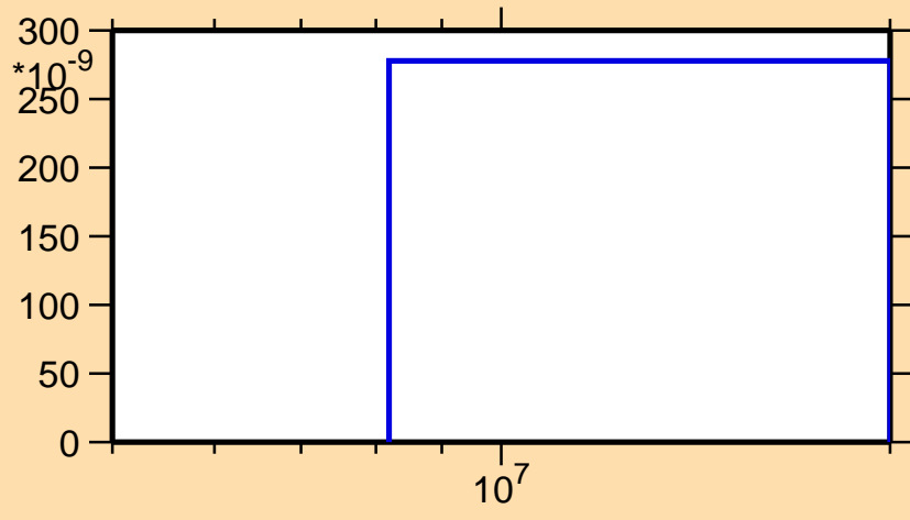
\sigma vs. E for ^{190}\text{Ta}(n,n\alpha)
