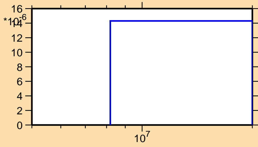
\sigma vs. E for ^{190}\text{Ta}(n,t)
