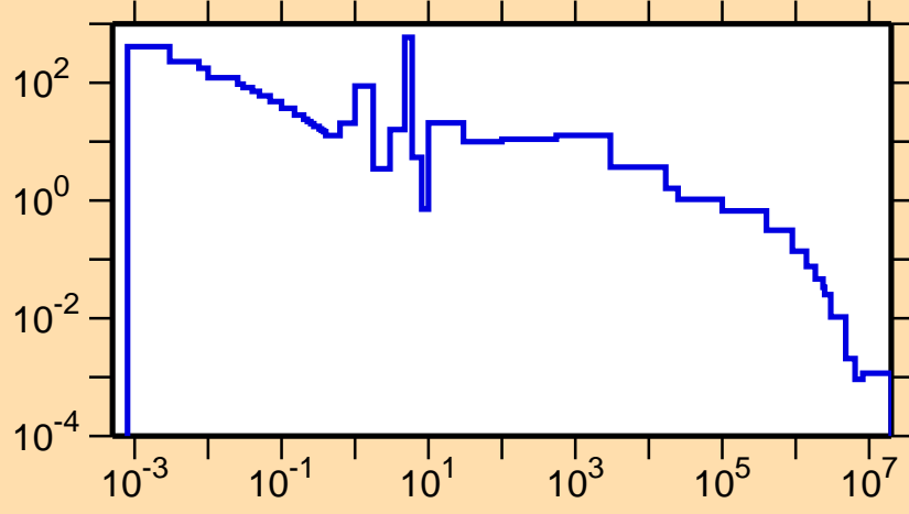
\sigma vs. E for ^{190}\text{Ta}(n,\gamma)
