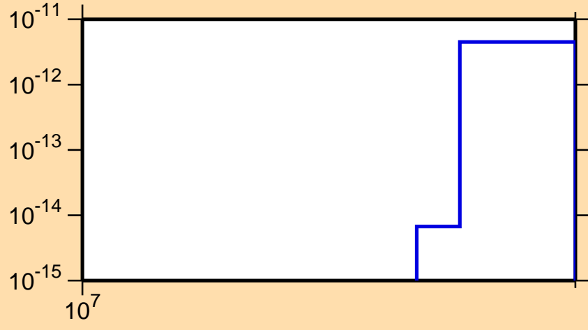
\sigma vs. E for ^{191}\text{Ta}(n,3n\alpha)
