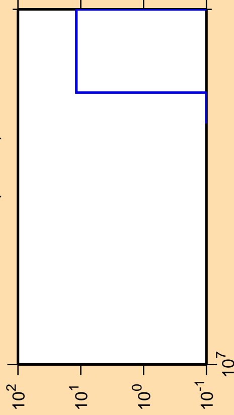
\Delta\sigma/\sigma vs. E for ^{191}\text{Ta}(n,3n\alpha)
