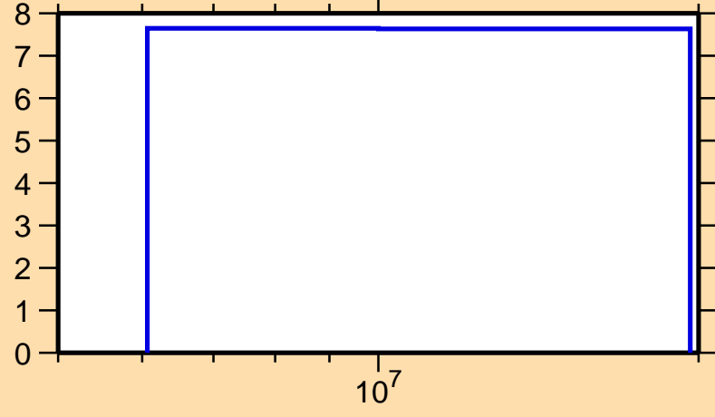
\Delta\sigma/\sigma vs. E for ^{191}\text{Ta}(n,\text{nonel.})
