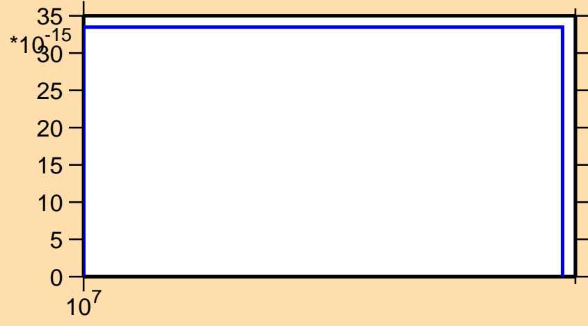
\sigma vs. E for ^{191}\text{Ta}(n,3n\alpha)
