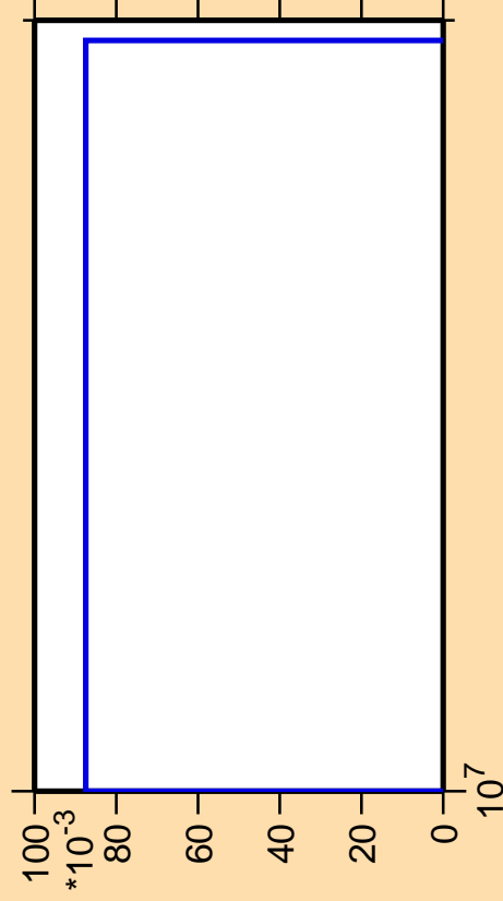
\Delta\sigma/\sigma vs. E for ^{191}\text{Ta}(n,3n\alpha)
