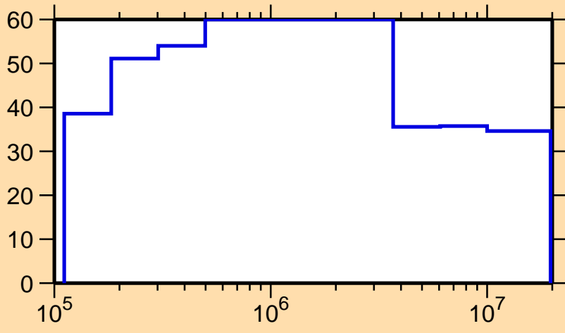
\Delta\sigma/\sigma vs. E for ^{191}\text{Ta}(n,n_1)
