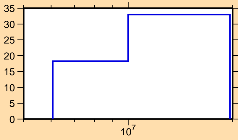
\Delta\sigma/\sigma vs. E for ^{191}\text{Ta}(n,2n)
