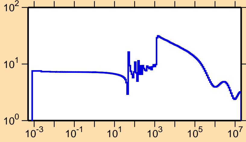
\sigma vs. E for ^{192}\text{Ta}(n,\text{el.})
