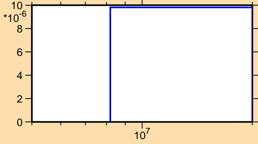
\sigma vs. E for ^{192}\text{Ta}(n,np)
