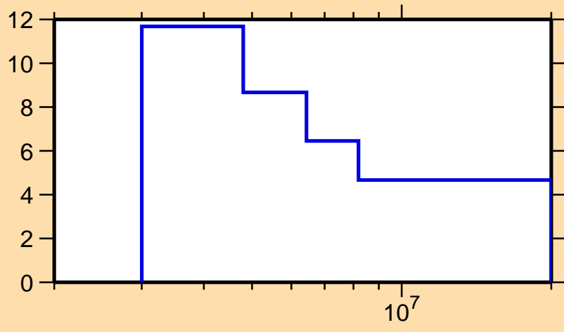
\Delta\sigma/\sigma vs. E for ^{192}\text{Ta}(n,\text{nonel.})
