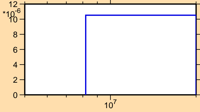
\sigma vs. E for ^{192}\text{Ta}(n,t)
