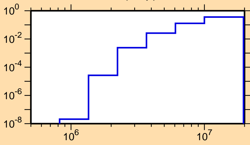
\sigma vs. E for ^{139}\text{Tb}(n,np)
