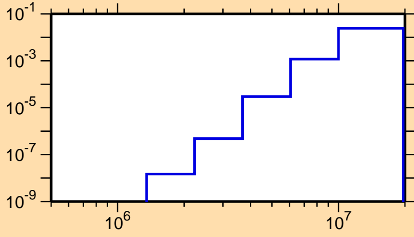
\sigma vs. E for ^{139}\text{Tb}(n,d)
