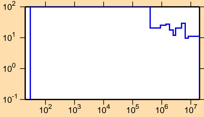
\Delta\sigma/\sigma vs. E for ^{139}\text{Tb}(n,\text{el.})
