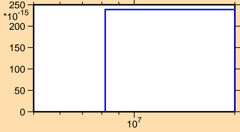
\sigma vs. E for ^{139}\text{Tb}(n,nt)
