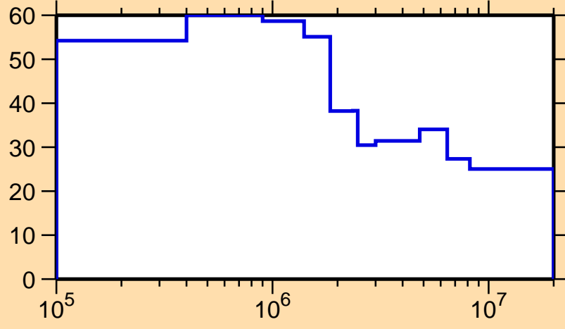
\Delta\sigma/\sigma vs. E for ^{139}\text{Tb}(n,n_1)
