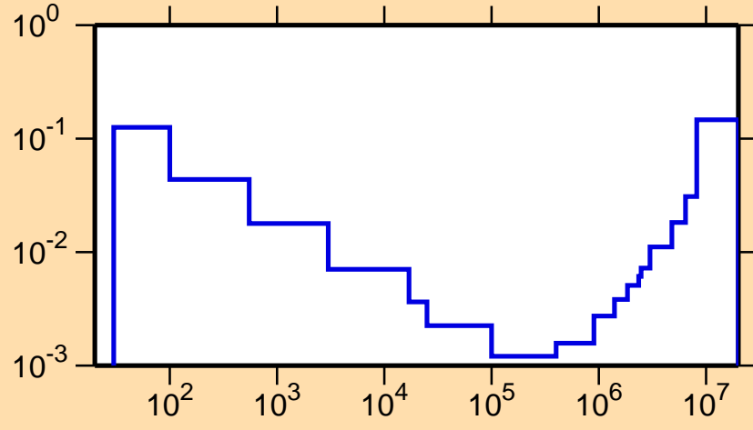
\sigma vs. E for ^{139}\text{Tb}(n,p\alpha)
