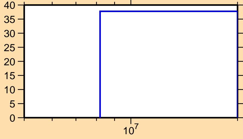
\Delta\sigma/\sigma vs. E for ^{139}\text{Tb}(n,\text{inel.})
