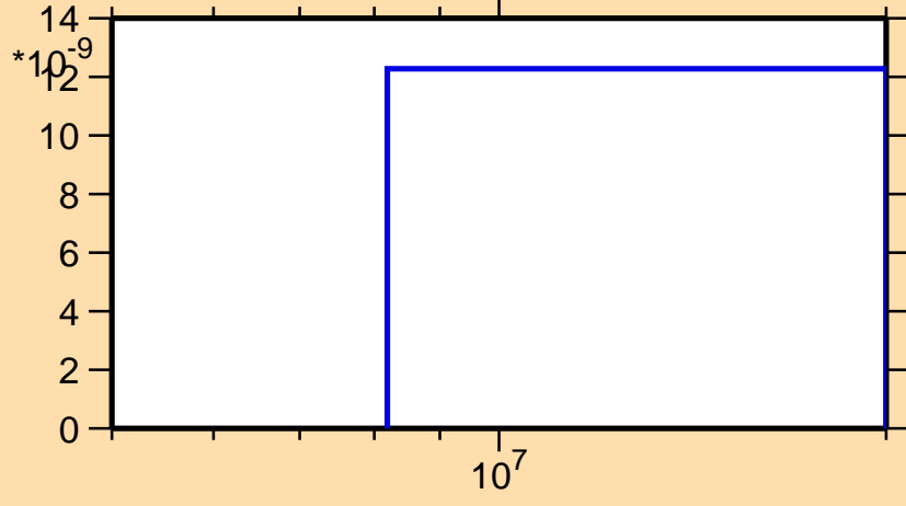
\sigma vs. E for ^{139}\text{Tb}(n,\text{nd})
