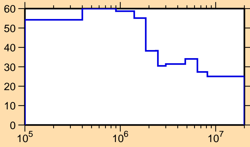
\Delta\sigma/\sigma vs. E for ^{139}\text{Tb}(n,n_1)
