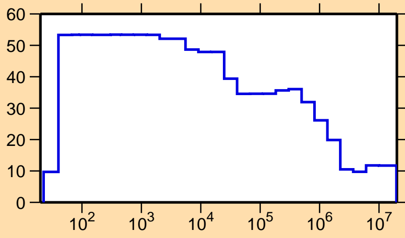
\Delta\sigma/\sigma vs. E for ^{140}\text{Tb}(n,\text{nonel.})
