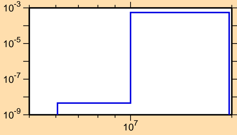
\sigma vs. E for ^{140}\text{Tb}(n,pd)
