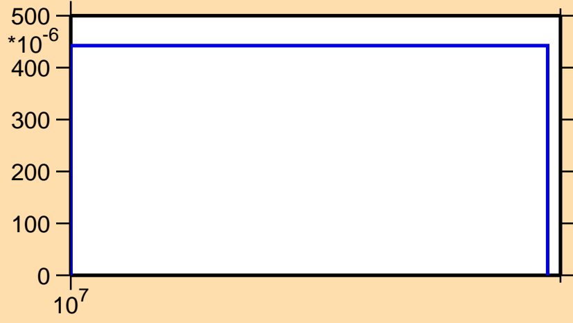
\sigma vs. E for ^{140}\text{Tb}(n,2n)
