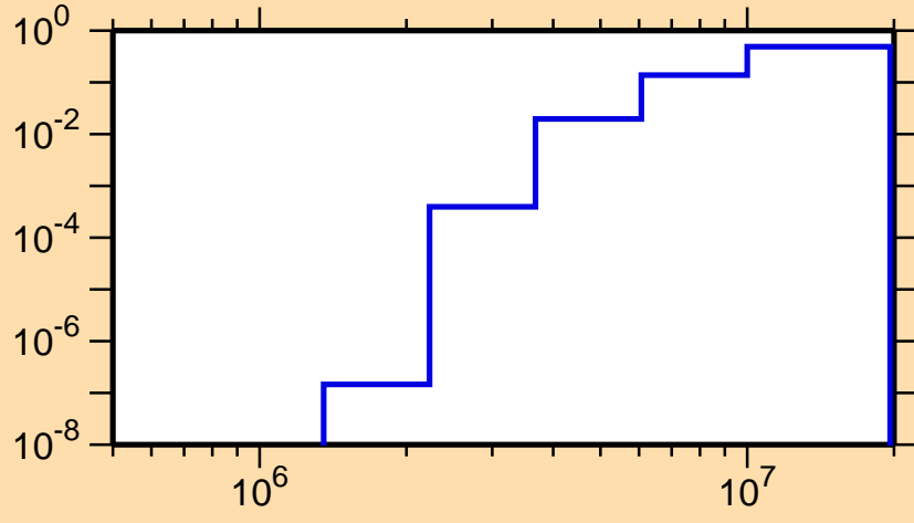
\sigma vs. E for ^{140}\text{Tb}(n,np)
