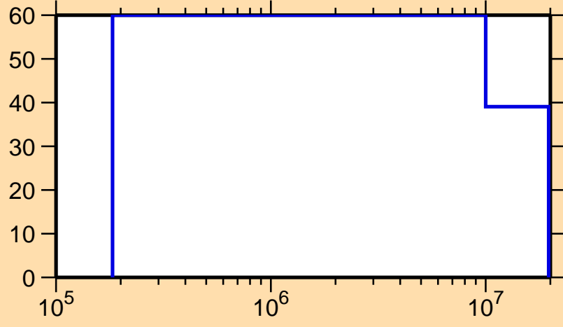
\Delta\sigma/\sigma vs. E for ^{140}\text{Tb}(n,n_1)
