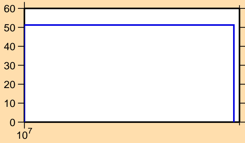
\Delta\sigma/\sigma vs. E for ^{140}\text{Tb}(n,2n)
