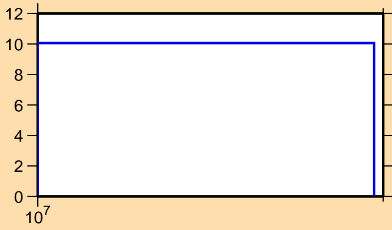
\Delta\sigma/\sigma vs. E for ^{140}\text{Tb}(n,\text{el.})
