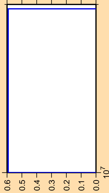
\Delta\sigma/\sigma vs. E for ^{140}\text{Tb}(n,nt)
