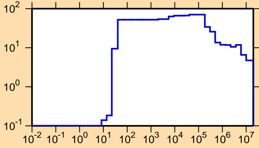
\Delta\sigma/\sigma vs. E for ^{140}\text{Tb}(n,\text{tot.})
