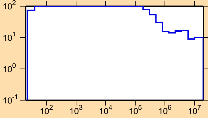
\Delta\sigma/\sigma vs. E for ^{140}\text{Tb}(n,\text{el.})
