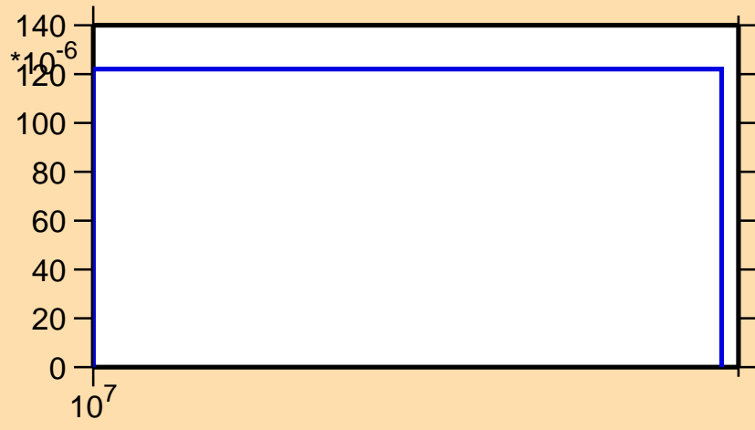
\sigma vs. E for ^{140}\text{Tb}(n,2np)
