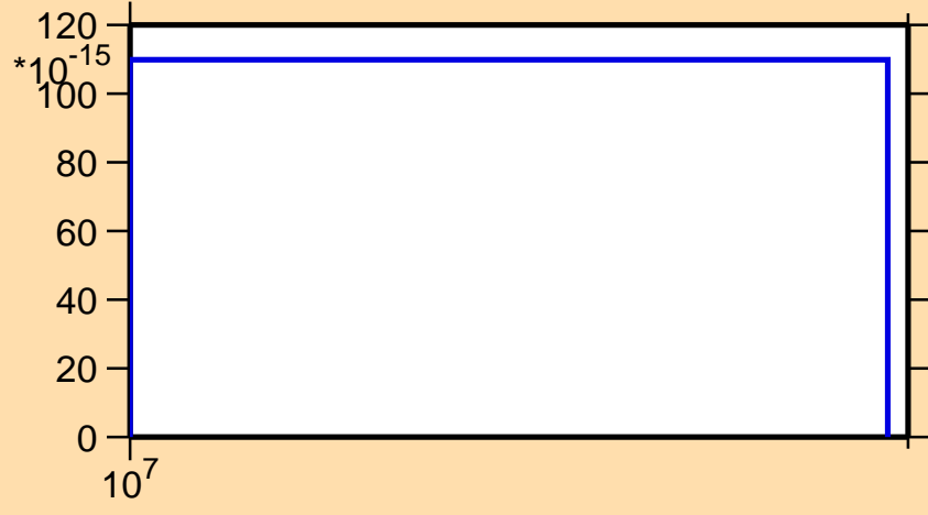
\sigma vs. E for ^{140}\text{Tb}(n,nt)
