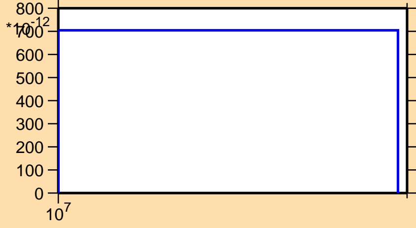
\sigma vs. E for ^{140}\text{Tb} (mt 34)
