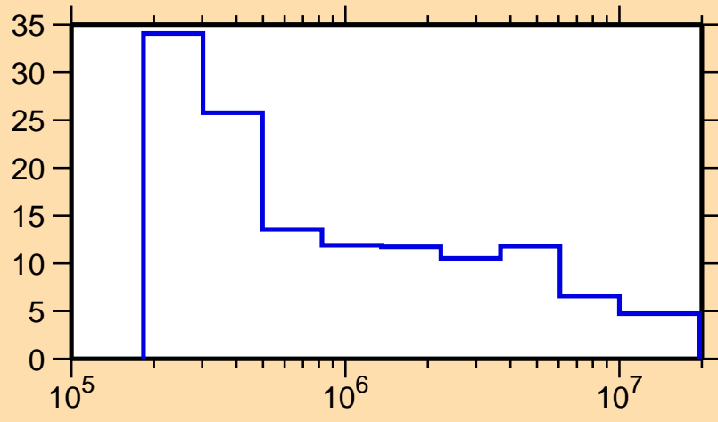
\Delta\sigma/\sigma vs. E for ^{140}\text{Tb}(n,\text{tot.})
