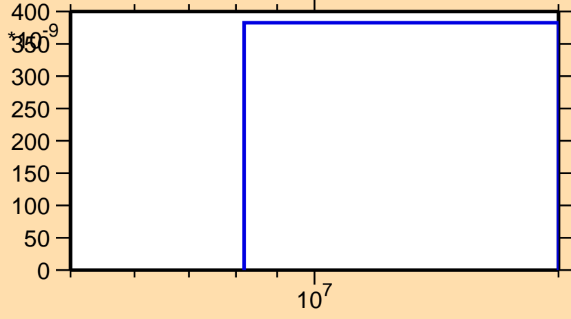
\sigma vs. E for ^{140}\text{Tb}(n,\text{nd})
