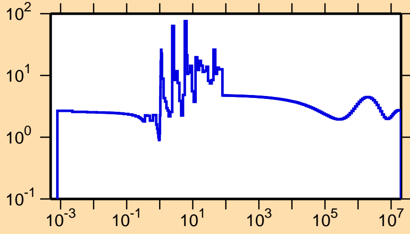
\sigma vs. E for ^{141}\text{Tb}(n,\text{el.})
