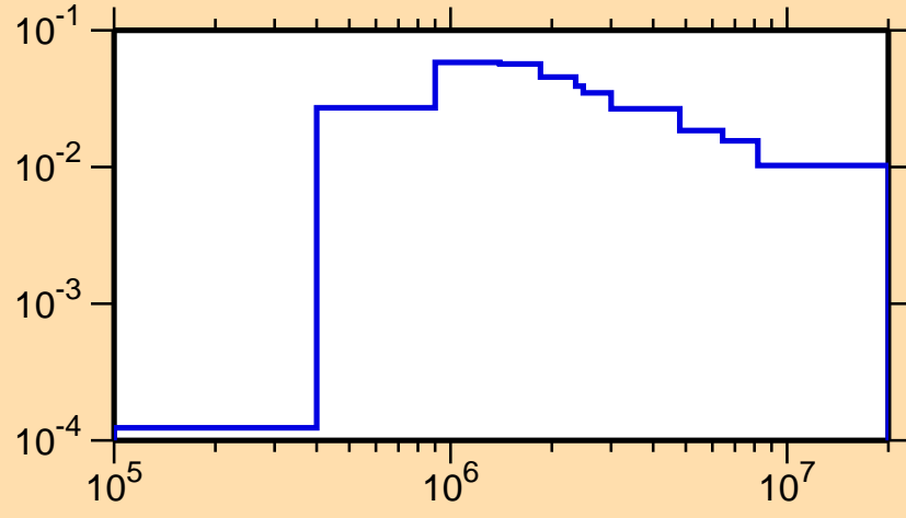
\sigma vs. E for ^{141}\text{Tb}(n,n_1)
