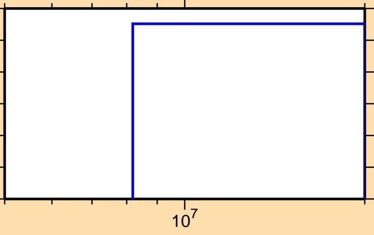
\sigma vs. E for ^{141}\text{Tb}(n,\text{pt})
