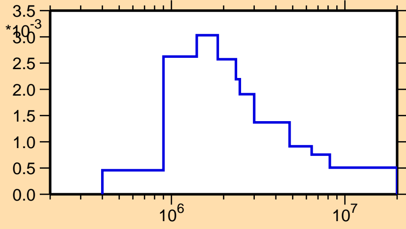
\sigma vs. E for ^{141}\text{Tb}(n,n_4)
