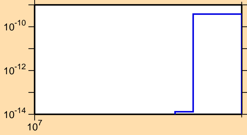
\sigma vs. E for ^{141}\text{Tb}(n,nt)
