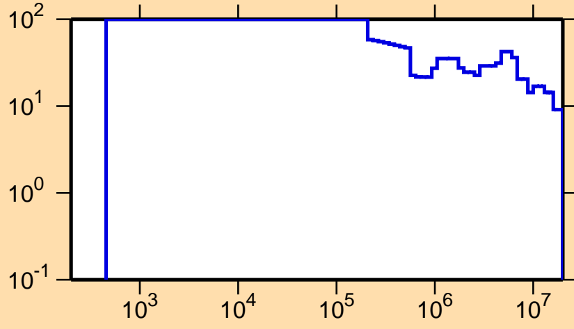
\Delta\sigma/\sigma vs. E for ^{141}\text{Tb}(n,\text{el.})
