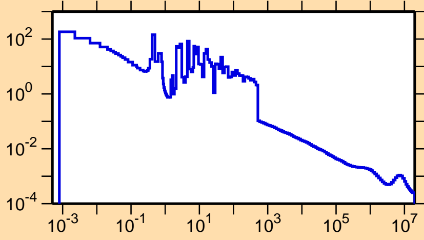
\sigma vs. E for ^{141}\text{Tb}(n,\gamma)
