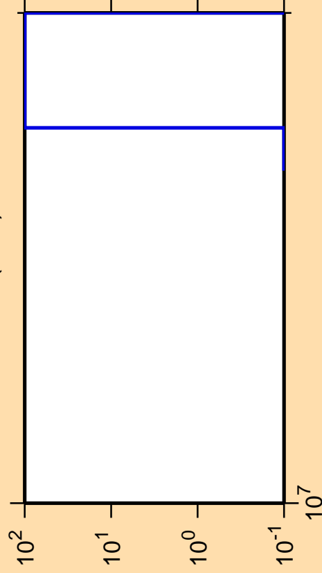
\Delta\sigma/\sigma vs. E for ^{141}\text{Tb}(n,nt)
