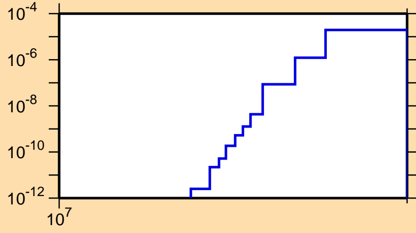
\sigma vs. E for ^{141}\text{Tb}(n,\text{pt})
