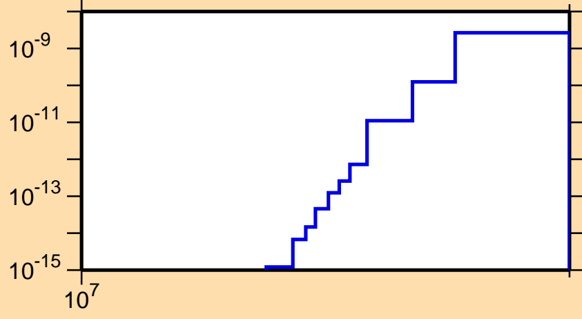
\sigma vs. E for ^{141}\text{Tb} (mt 34)
