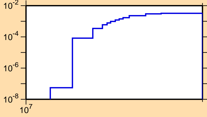
\sigma vs. E for ^{141}\text{Tb}(n,2n)
