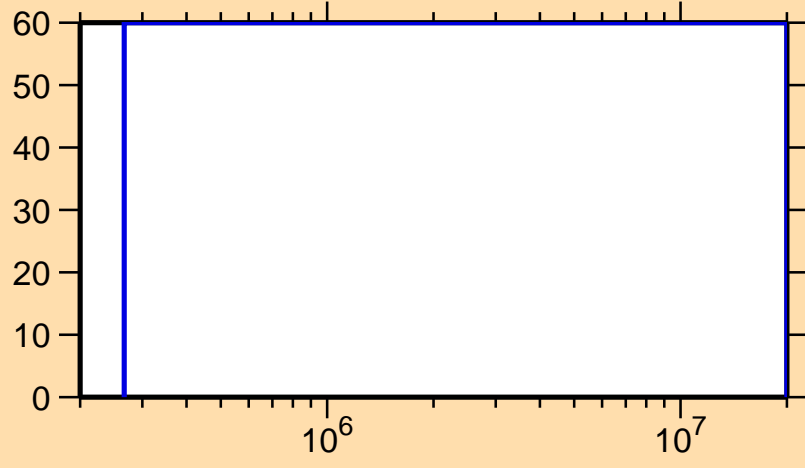
\Delta\sigma/\sigma vs. E for ^{141}\text{Tb}(n,n\text{cont.})
