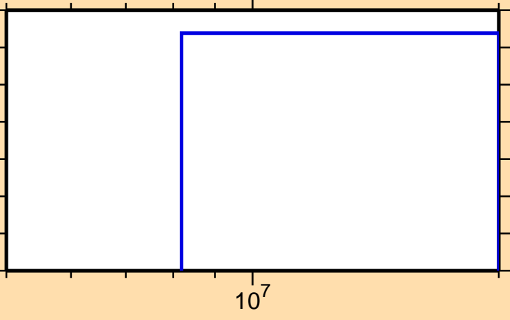
\sigma vs. E for ^{141}\text{Tb}(n,2np)
