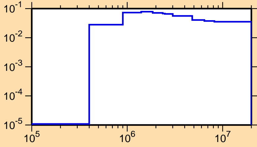
\sigma vs. E for ^{141}\text{Tb}(n,n\text{cont.})
