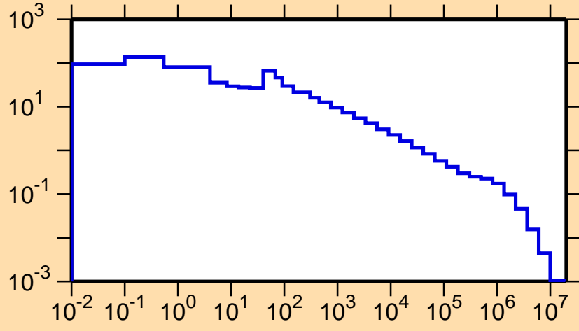
\sigma vs. E for ^{143}\text{Tb}(n,\gamma)
