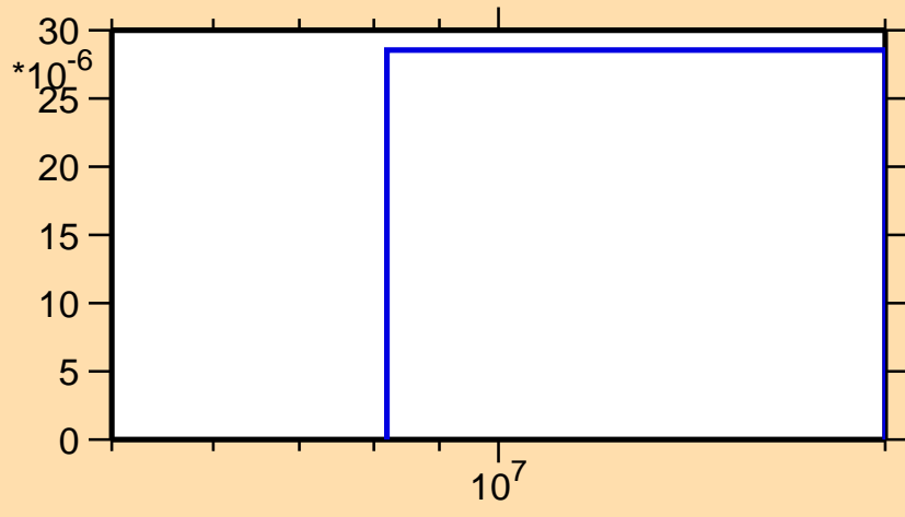
\sigma vs. E for ^{143}\text{Tb}(n,pd)
