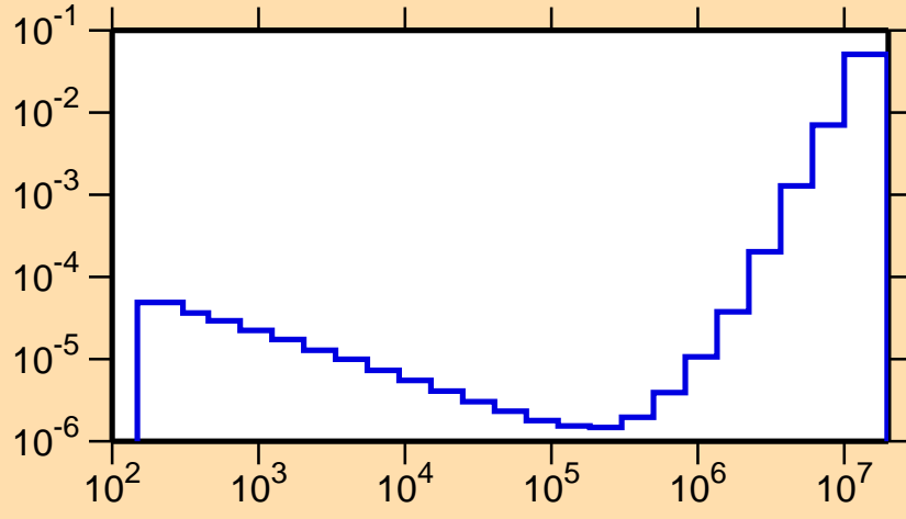
\sigma vs. E for ^{143}\text{Tb}(n,p\alpha)
