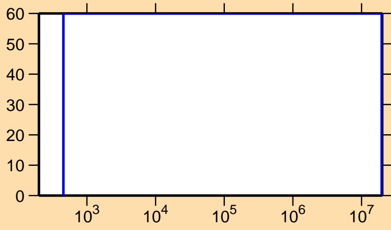
\Delta\sigma/\sigma vs. E for ^{143}\text{Tb}(n,n_1)
