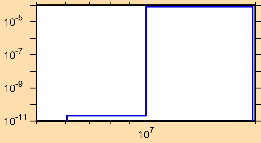
\sigma vs. E for ^{143}\text{Tb}(n,\text{pd})
